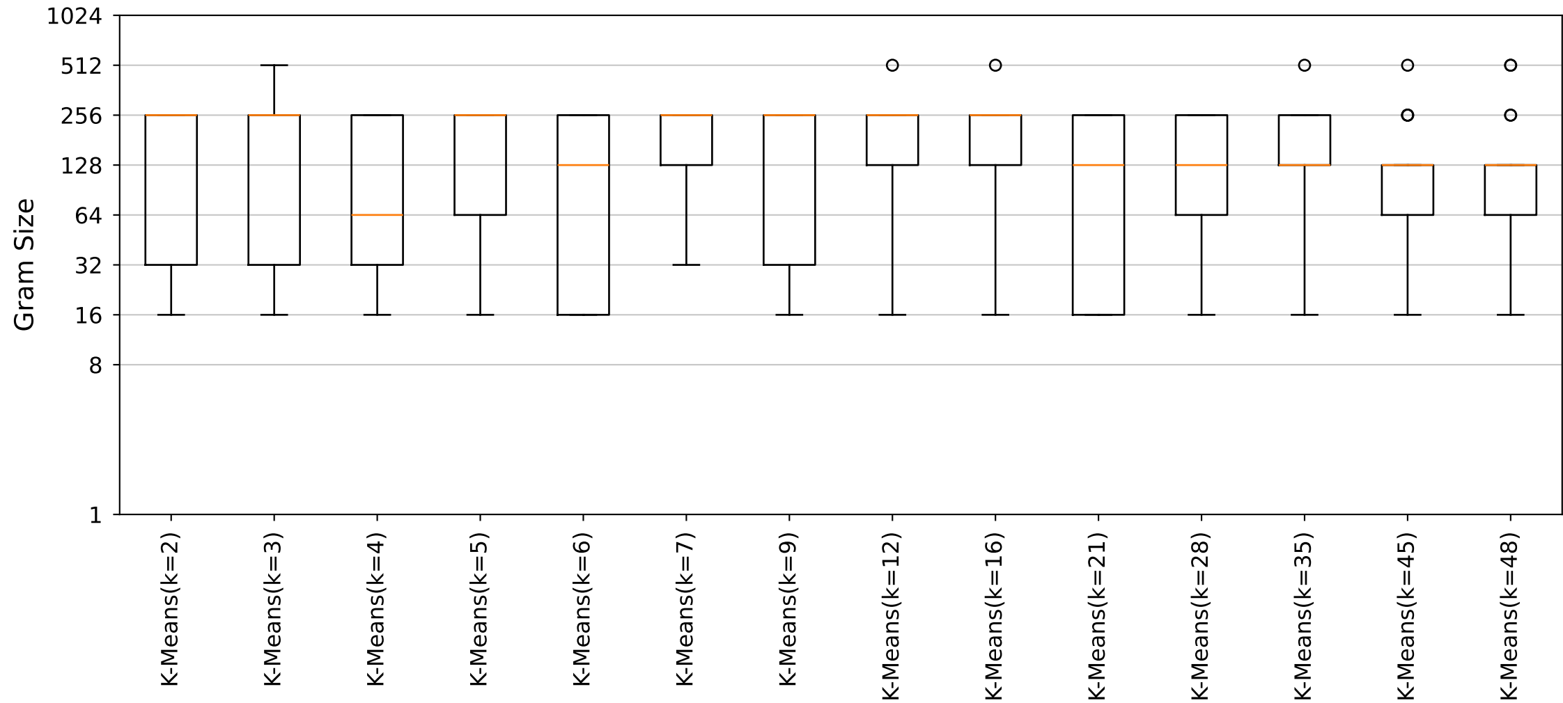
YARA Rules Gram Size Distribution (Cluster4_Size48 dataset)
